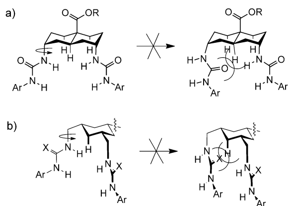
Figure 2. a) Conformational restrictions in diureidodecalins 2 . Rotation about the axial C–N bonds is strongly disfavored by steric interactions with axial CH. Intramolecular H-bonding is thus disallowed. b) Similar restrictions apply in 3 and 4 . Attempts to form intramolecular H-bonds are prevented by axial CH.
